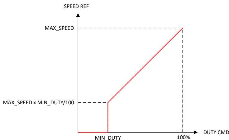
Figure 7-13. Speed Input Transfer Function
