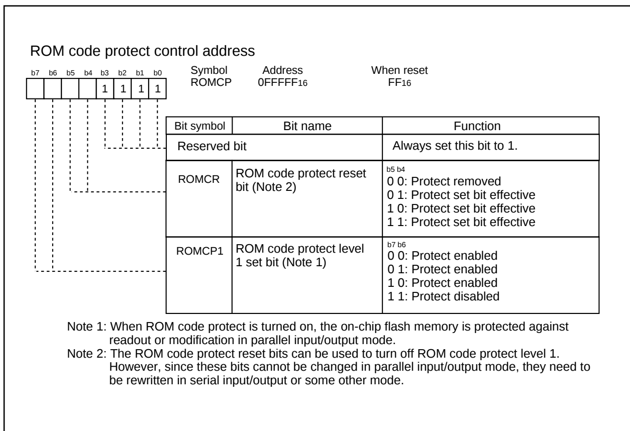
Figure 1.30.1. ROM code protect control address
